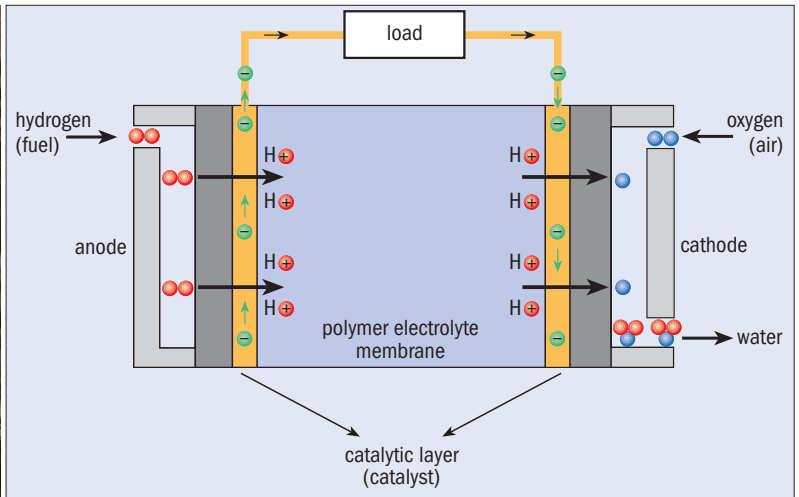
Bubbling away A fuel cell generates electricity by reacting oxygen, hydrogen ions and electrons (artist's impression, left). The hydrogen ions generated at the anode are swept through a membrane to the cathode. The membrane is often made from a polymer called Nafion, which has a Teflon skeleton with negatively charged groups of sulphur trioxide attached to it. This membrane is impermeable to electrons generated at the anode, which are routed to the cathode via an external circuit that is powered by the cell.
