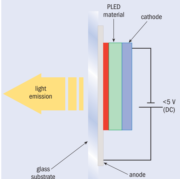
The polymer LED (PLED) has a simpler structure than a conventional LED, consisting of a thin layer of polymeric semiconducting material sandwiched between two metal electrodes. When a voltage is applied, the polymer glows and the light is emitted through the anode, which is transparent.
