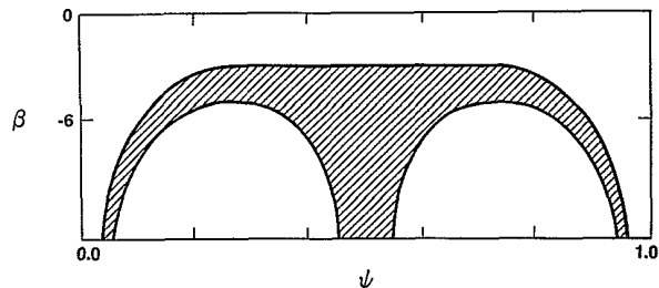
FIG. 1. Range of interaction strength where vesicles are stable (shaded area) as a function of the relative composition \psi . The figure is drawn for the case where the spontaneous curvatures of the two surfactants are positive (tending to make micelles in oil), c_1 = c_2 = 1/2\delta , where \delta is of order the surfactant size.
