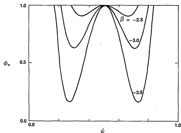
FIG. 2. Stability boundary for the vesicle phase as a function of the composition asymmetry \psi and the water volume fraction \phi_w . Curves are shown for three values of the interaction parameter \beta . The figure is drawn for the case where the spontaneous curvatures of the two surfactants are positive (tending to make micelles in oil), c_1 = c_2 = 1/2\delta , where \delta is of order the surfactant size.
